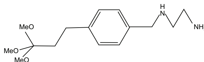
(Aminoethylaminomethyl)phenethyltrimethoxysilane
