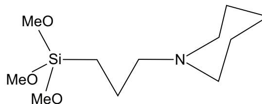
3-Piperidinopropyltrimethoxysilane
