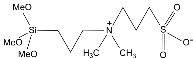
N-(3-(Trimethoxysilyl)propyl)dimethylammoniopropylsulfonate
