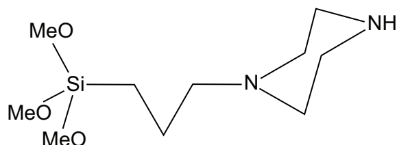
3-Piperazinopropyltrimethoxysilane
